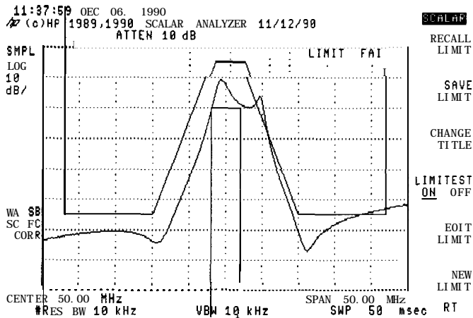
limit line with LIMIT FAIL message
