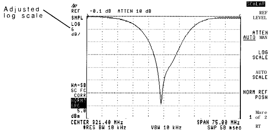
Response after Automatic Scaling
