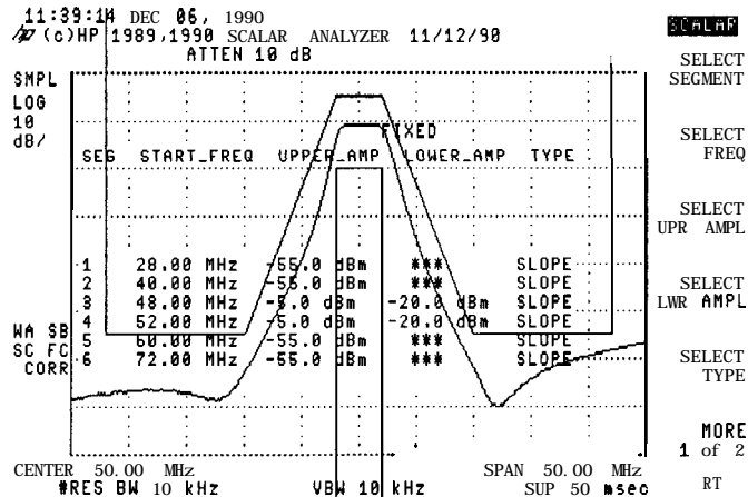
Upper/lower limit lines
