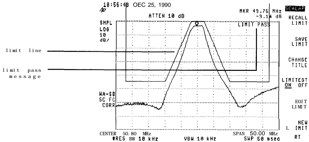
limit line with LIMIT PASS message
